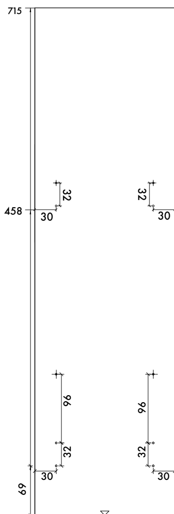
FRONT FIXING POSITIONS
