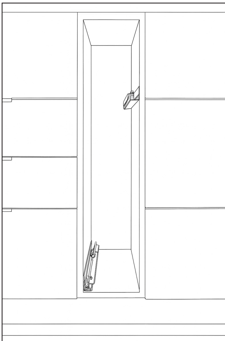
LEGRABOX 150 pull-out runner positions
